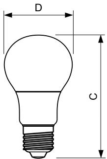
Entry bulb 6.5W-45W 470lm150D 2700K E27D
