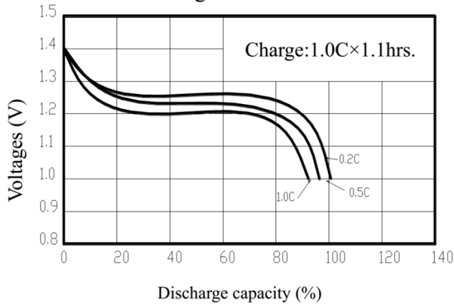
Discharge characteristics
